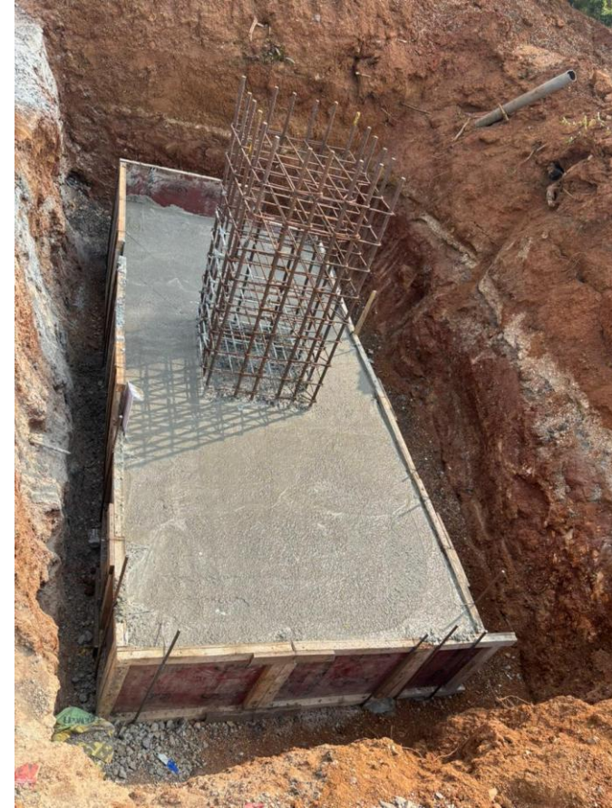
Construction of Footings for Gantry at Hyderabad International Airport Main Access Road (GMR Work)
